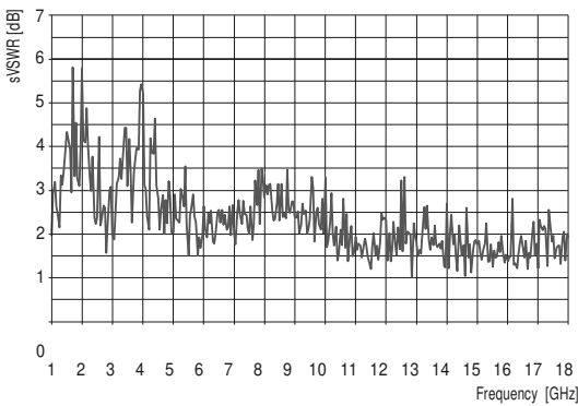
Typical performance Automotive 5 m (sVSWR)
