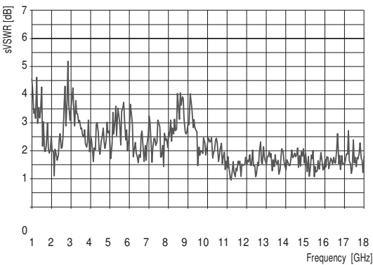
Typical performance Automotive 10 m (sVSWR)
