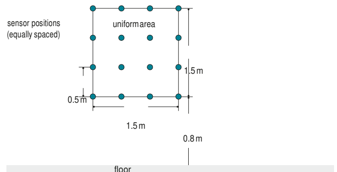
Uniform area for field uniformity test
