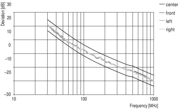
Typical performance Automotive 5m (NSA)
