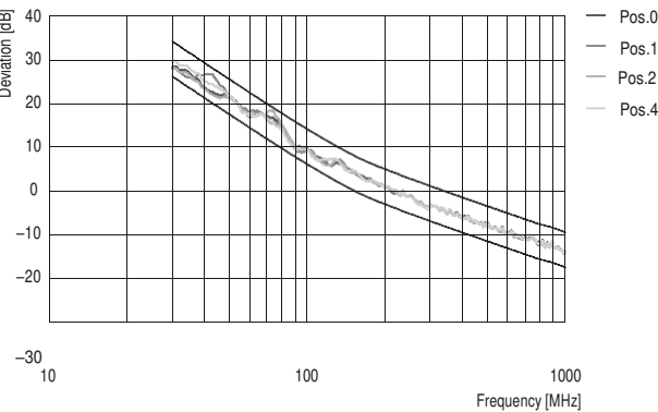
Typical performance Automotive 10 m (NSA)
