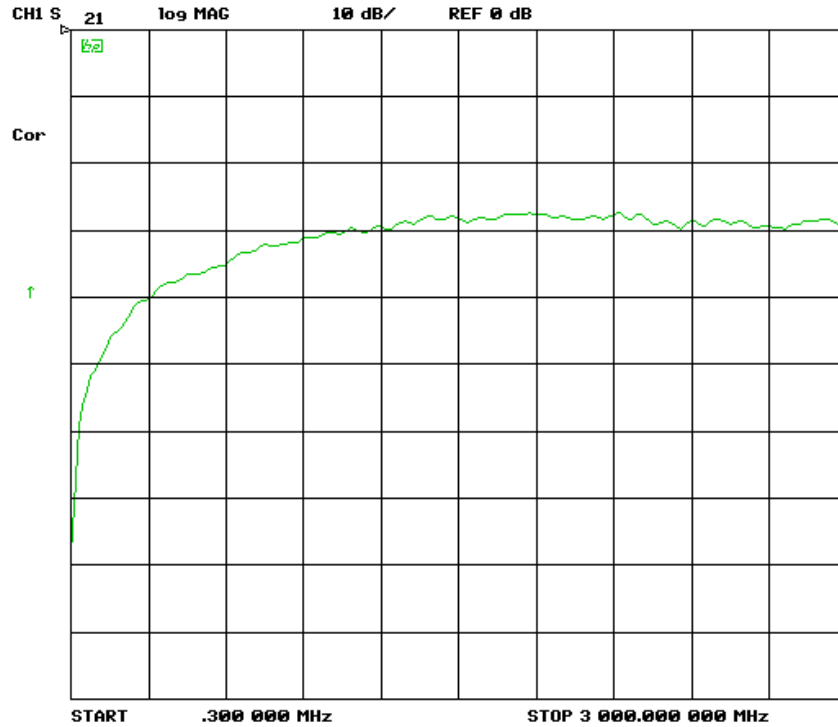
Picture 9 – H5, coupling loss, 300 kHz – 3 GHz
